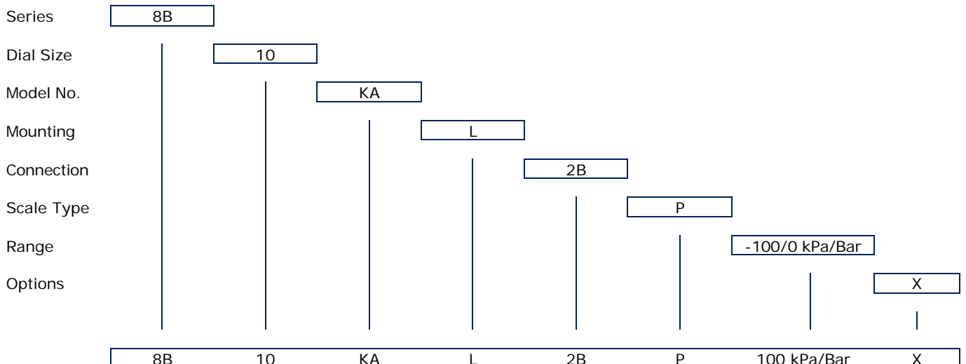
Series8 Brass wetted parts, 100mm, Bottom Entry, 1/2" BSP Parallel, Vacuum -100/0 kPa / Bar Dual Scale
